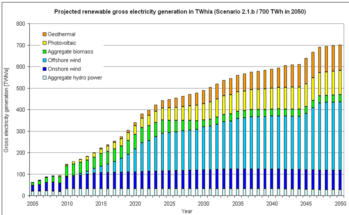
Projected renewable gross electricity generation in TWh/a (scenario 2.1.b/700 TWh in 2050)
